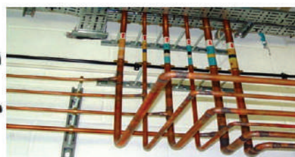
Medical Gas Pipeline System
